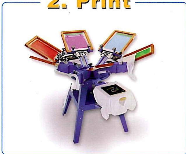
V6100 6 color 1 station printer
